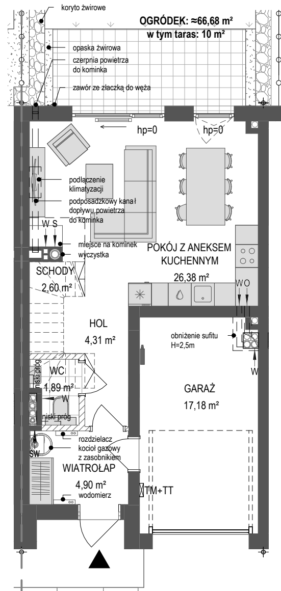
PARTER 57,26 m 2
